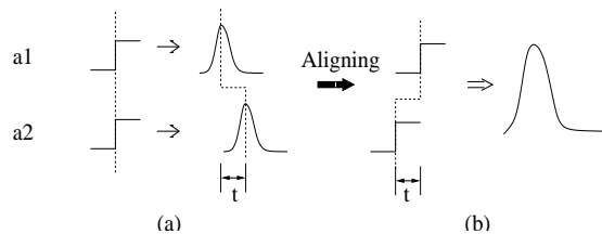
Fig. 1. Alignment operation illustrated using two aggressors. (a) We simulate the interconnects with only one aggressor switching in each simulation, and find the skew t between noise peaks. (b) We simulate the interconnects with both aggressors switching. When their switching times are aligned by t , the overall noise due to the two aggressors is likely maximized [1].
