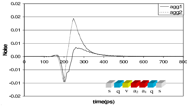
Fig. 3. noises on the victim caused by two aggressors in a five-bit 1000\mu\text{m} -long bus. The driver size is 30\times , and the wire spacing is 1.7\mu\text{m} .
