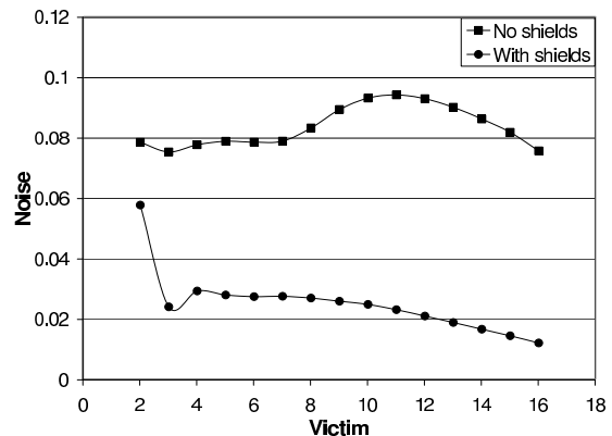
Fig. 2. Noise in a sixteen-bit 1000 \mu m-long bus. The driver size is 200 \times , and the wire spacing is 0.6 \mu m
