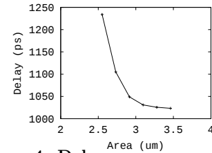
Figure 4: Delay-area curve of C499
