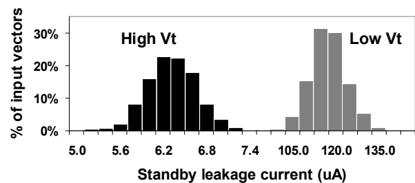
Fig. 12: Leakage control by natural stacks
