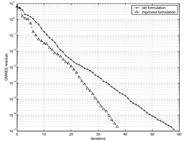
Figure 11: GMRES residual in old and improved formulation, a multipin connector
