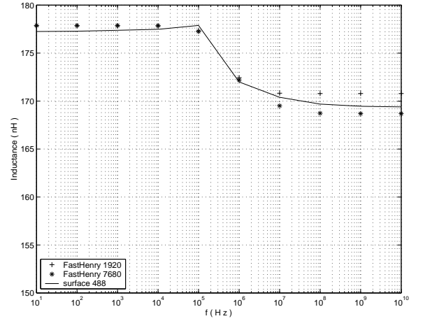
Figure 9: Inductance of a spiral
