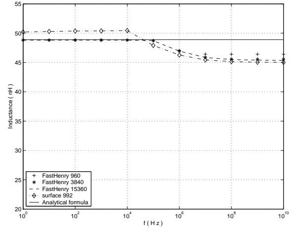
Figure 7: Inductance of a ring
