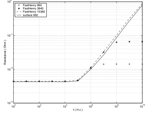
Figure 6: Resistance of a ring
