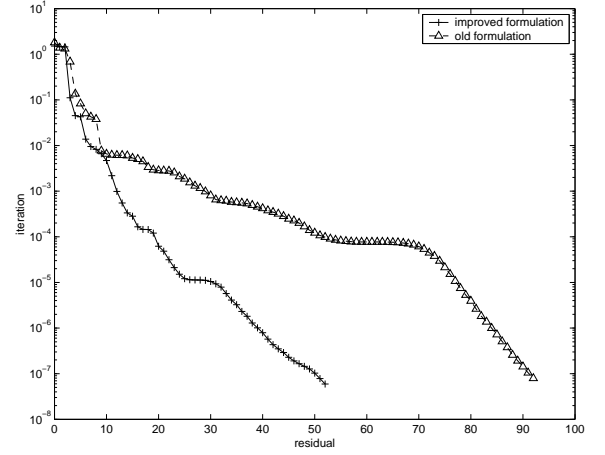
Figure 10: GMRES residual in old and improved formulation, a spiral inductor over ground plane
