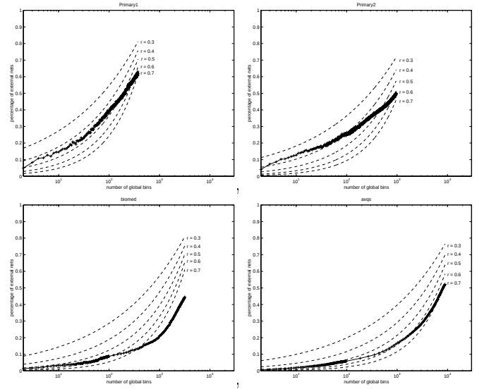
Figure 2: Percentage of external nets vs. number of global bins.
