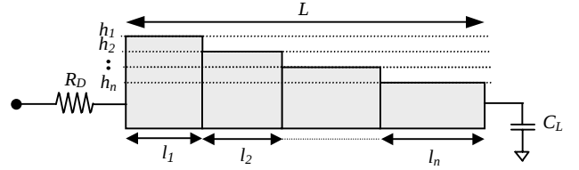
Figure 3. The wire sizing (WS) problem for a single interconnect wire.
