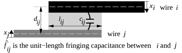
Figure 4: Two neighboring wires has coupling capacitance.
