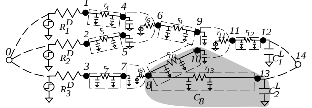
Figure 3: A circuit is transformed to an RC network. As an example, the delay D_8 = r_8 C_8 , where C_8 is the sum of all the capacitors in the shaded area.
