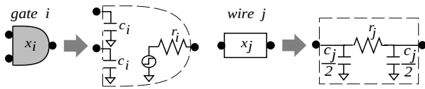
Figure 2: A gate/wire is modeled as a combination of RC elements. A gate is the loading of its upstream, but the driver of its downstream. A wire is represented by the \pi model.
