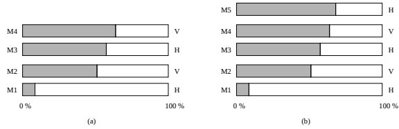
Figure 4: Difference between the available track length in the horizontal and vertical directions. The second topmost layer defines the direction which is most congested.
