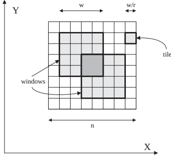
Figure 1: The layout is partitioned using r^2 ( r = 4 ) distinct dissections (each with window size w \times w ), into \frac{nr}{w} \times \frac{nr}{w} tiles. Each w \times w window (darker) consists of r^2 tiles. Note that a pair of windows from different dissections may overlap.
