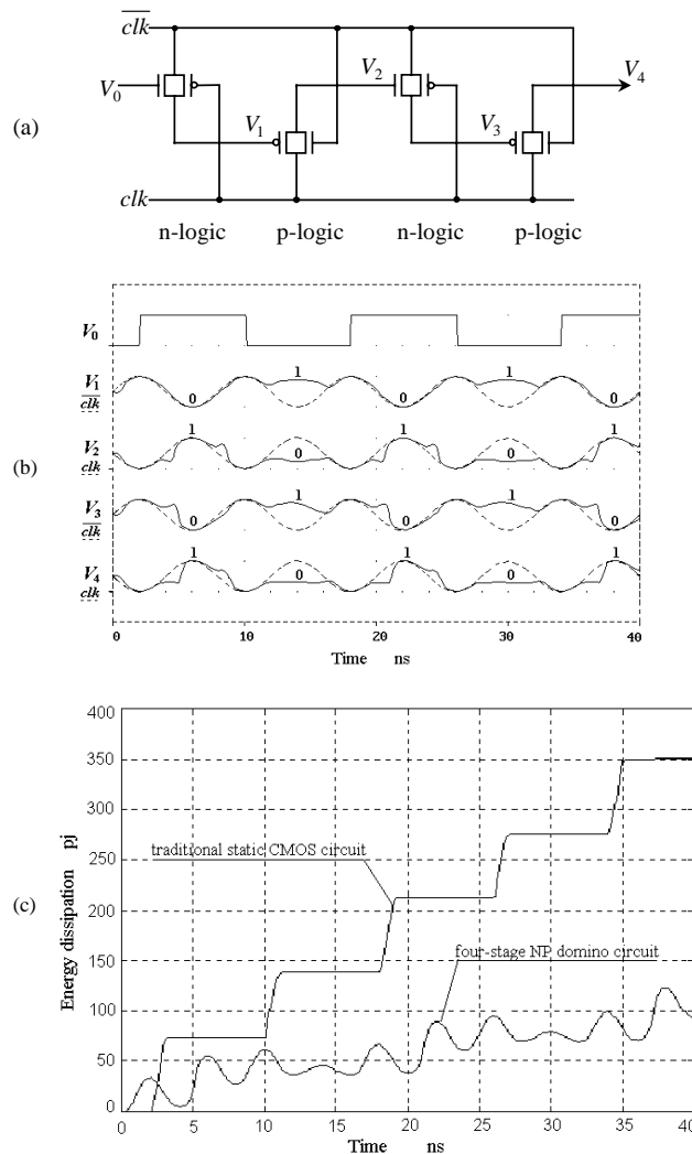
Figure 8 Simulation of four-stage NP domino circuit using a sinusoidal power-clock.
