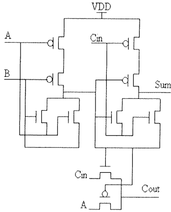
Figure 4. The New Static Energy-Recovery Full (SERF) Adder
