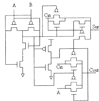
Figure 2. The dual value logic (DVL) adder [7]
