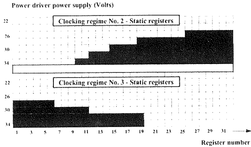
Fig. 10. Noise tolerance affecting specific register location as a function of power driver voltage, substrate bias, clocking regime, ground bias, and active power driver group. Group 2 is active. Black shaded area represents the affected registers.
