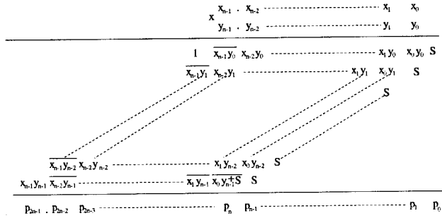
Figure 2. Saturating Multiplication.
