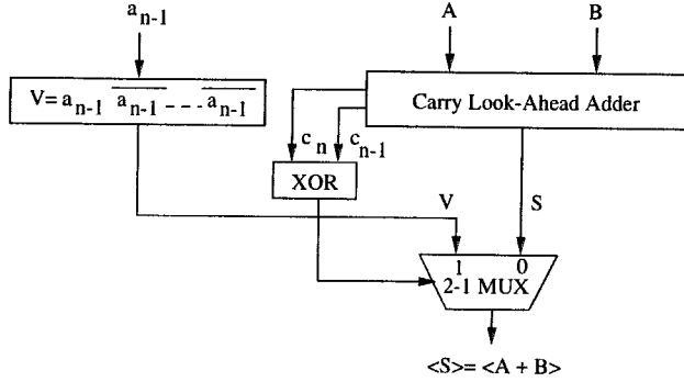
Figure 4. Saturating Adder.
