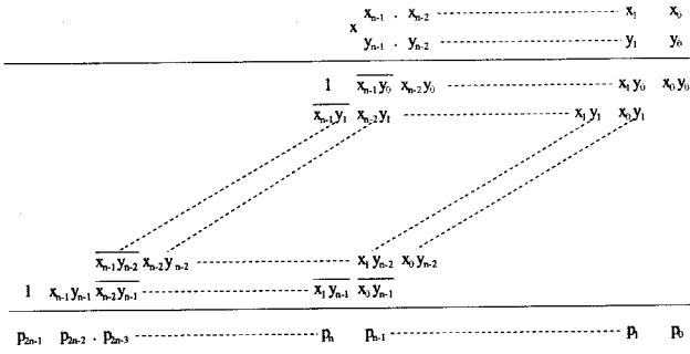
Figure 1. Non-Saturating Multiplication.
