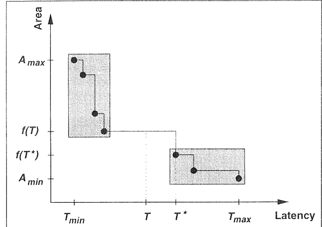
Figure 1: Example design space showing Pareto points. The shaded regions show the two distinct clusters of Pareto points that many tradeoff curves exhibit.
