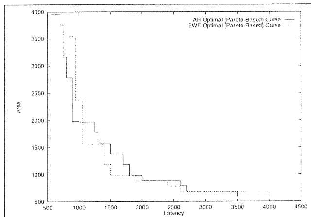
Figure 4: The EWF and AR optimal Pareto-base curves when using the library from Table 5
