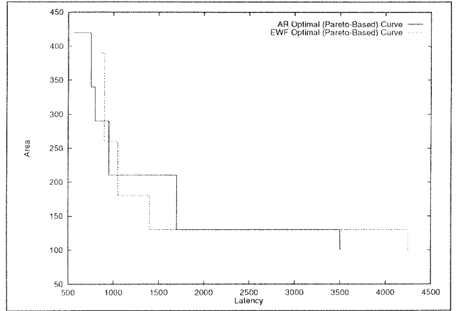
Figure 3: The EWF and AR optimal Pareto-base curves when using the library from Table 1
