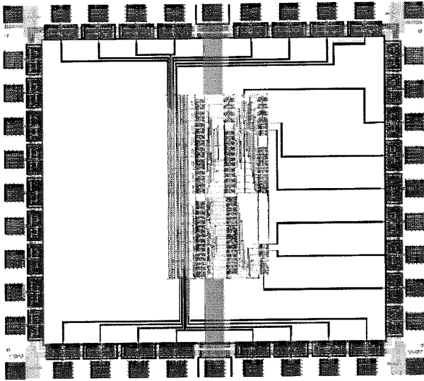
Fig. 4. VLSI Layout of the chip in 2-μm n-well CMOS technology.
