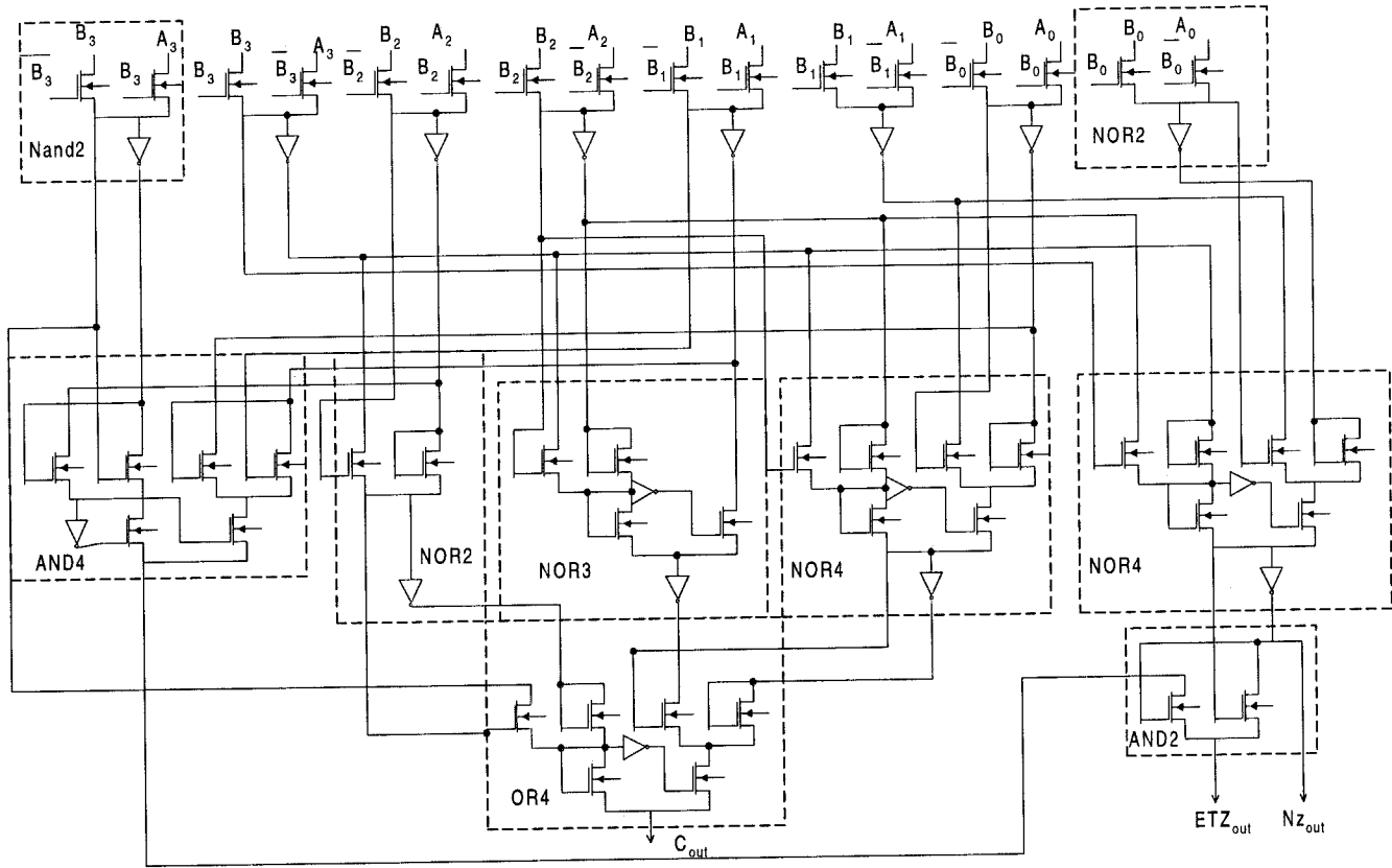
Fig. 2. Transistor level schematic diagram of the 4-bit fast carry and equal to zero detector.
