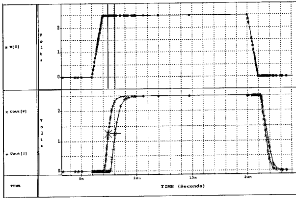
Fig. 5. HSPICE Simulation results of the chip, top input, and bottom Cout[P] (proposed, legend*) and Cout[I](legend +).
