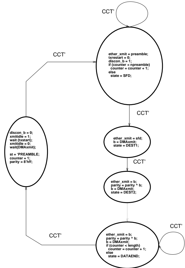
Figure 4. Program state machine for process xmit_frame
