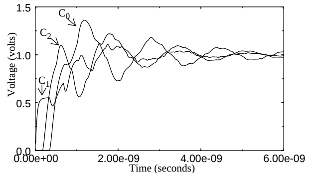
FIGURE 7: Time-domain waveforms for example in Fig.6 with unit step input.
