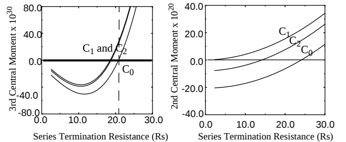
FIGURE 6: Third and second central moment vs. series termination resistance, R_s , for three drop net with source at C_1 .
