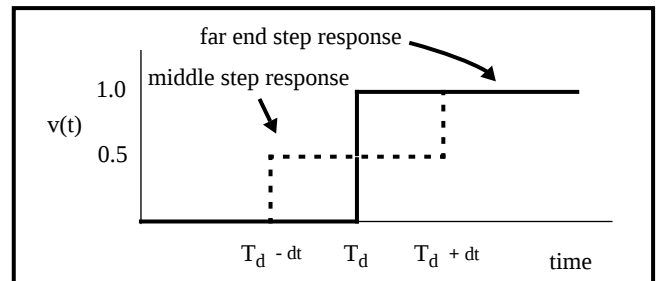
FIGURE 2: Ideal middle and far end step response.
