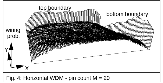
Fig. 4: Horizontal WDM - pin count M = 20
