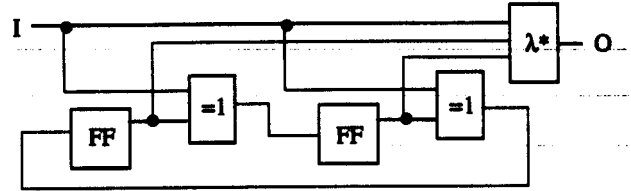
Figure 6: Structure of M^* .
