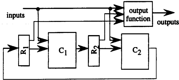
Figure 3: Controller target structure.
