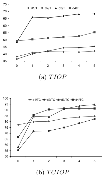
Figure 4: Comparison of CSR. The x -axis is the iteration number and the y -axis is CSR in percentage, with CIOP 's CSR being 100%.
