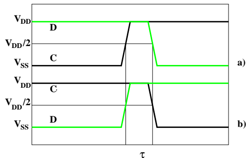
Figure 4: Possible input waveforms of the gate G of Fig. 4 giving rise to an output static hazard.
