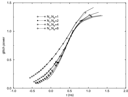
Figure 11: Glitch power as a function of the skew for asymmetric input loading and fan-out = 2.
