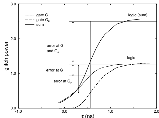
Figure 14: Glitch power dissipated at gate G , G_P and their sum as a function of the skew as compared with that evaluated in logic simulation.
