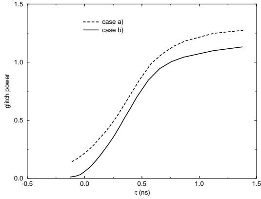
Figure 6: Glitch power dissipated for two different sequences of input stimuli ((a) and (b)) in a CMOS NAND gate.
